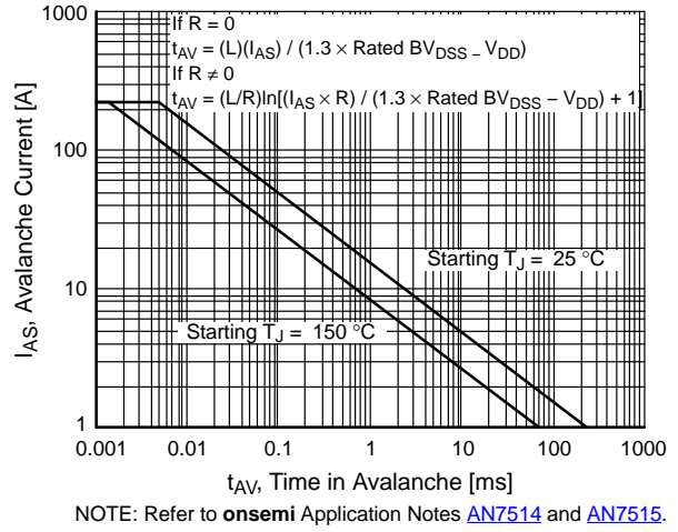
Figure 6. Unclamped Inductive Switching Capability
