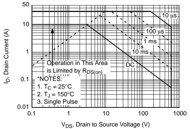
Figure 10. Maximum Safe Operating Area for FCPF380N60
