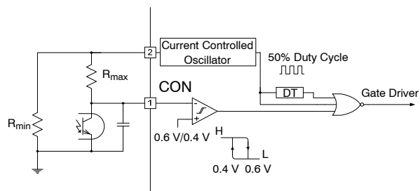
Figure 42. Pulse-Skipping Circuit
