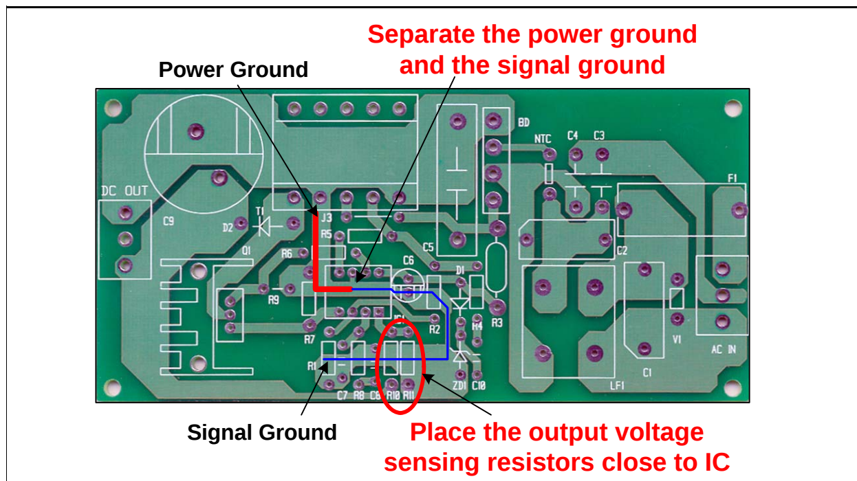
Figure 39. PCB Layout Considerations for FAN7529
