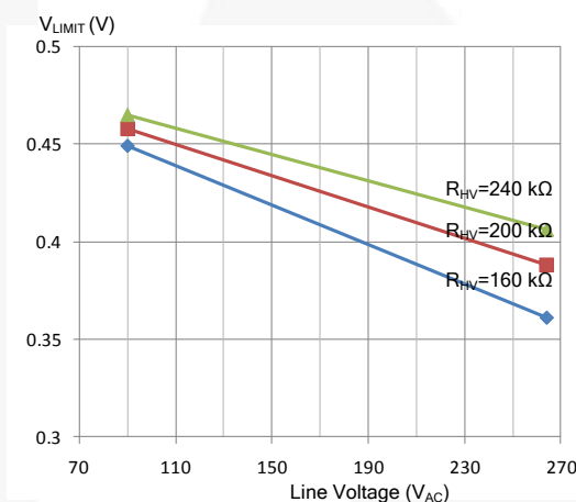
Figure 26. Current Limit vs. Line Voltage
