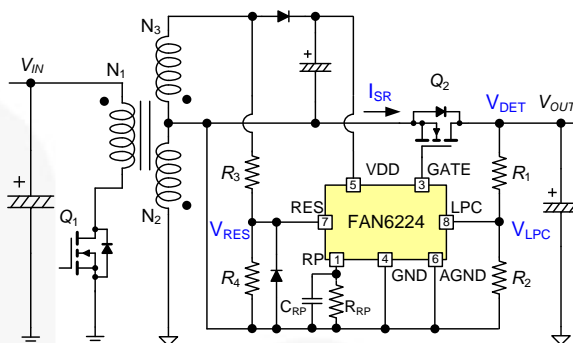
Figure 2. Flyback High-Side SR
