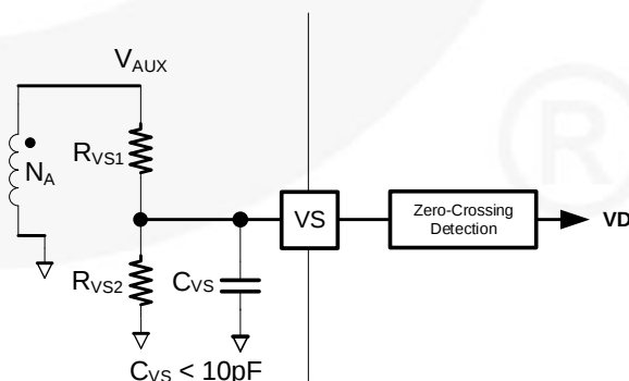
Figure 26. The Valley Detection Circuit
