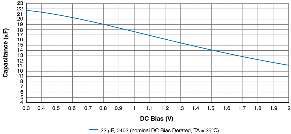
Figure 35. Typical 22 \mu\text{F} Ceramic Capacitor Value vs. DC Bias Voltage
