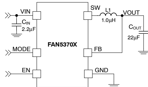
Figure 1. Typical Application
