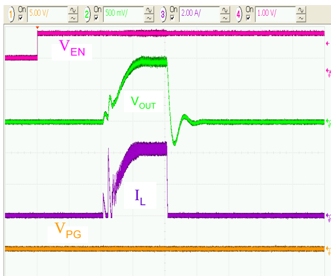
Figure 25. Over-Current at Startup, R_{LOAD}=200\text{ m}\Omega , 50 \mu\text{s}/\text{div} .
