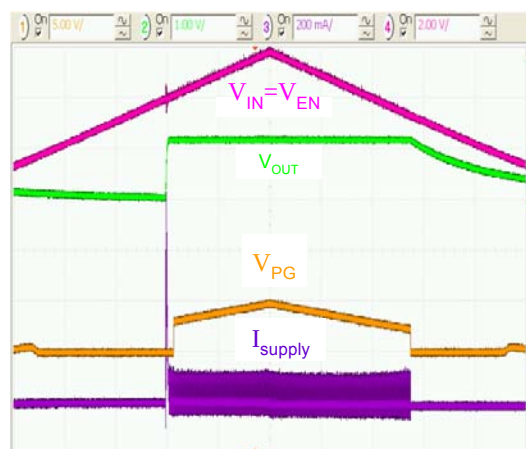
Figure 18. Soft-Start, EN Pin Tied to VCC I_{LOAD}=0 , 1 ms/div.
