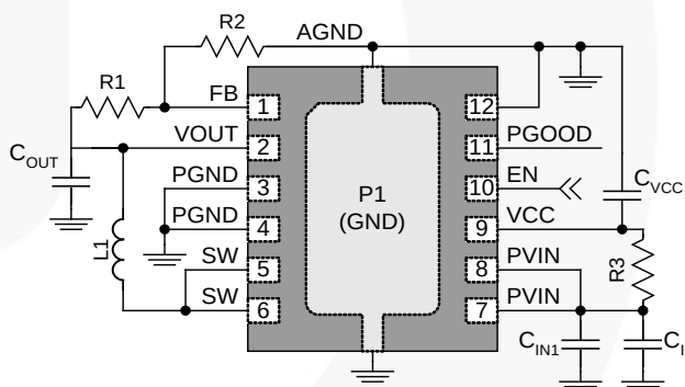
Figure 1. Typical Application
