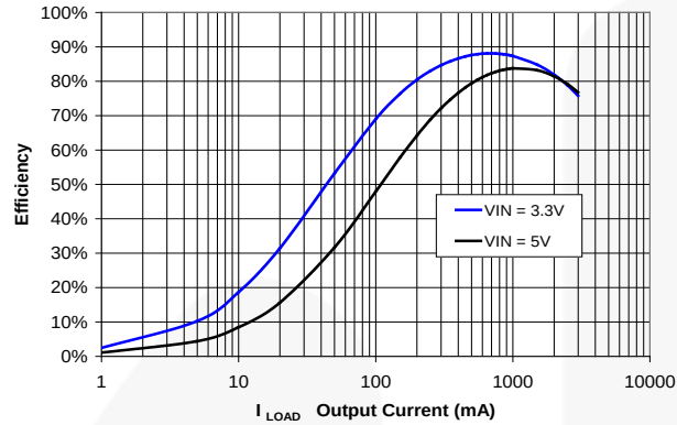
Figure 3. Efficiency vs. I_{LOAD} at V_{OUT} = 1.2\text{ V}
