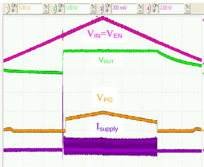
Figure 16. Soft-Start: EN Pin Tied to VCC, I_{LOAD} = 0 , Horizontal Scale = 1\text{ ms/div} .
