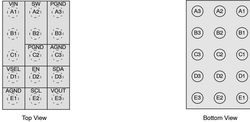
Figure 2. Pin Configuration
