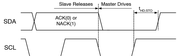
Figure 20. STOP Bit
