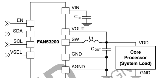
Figure 1. Typical Application
