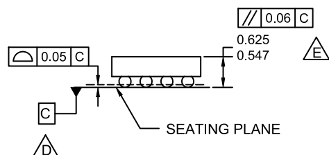
SIDE VIEWS
