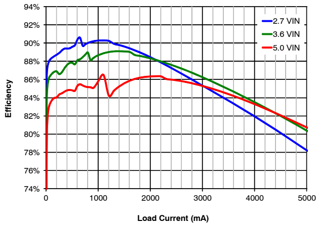
Figure 3. Efficiency vs. Load Current and Input Voltage
