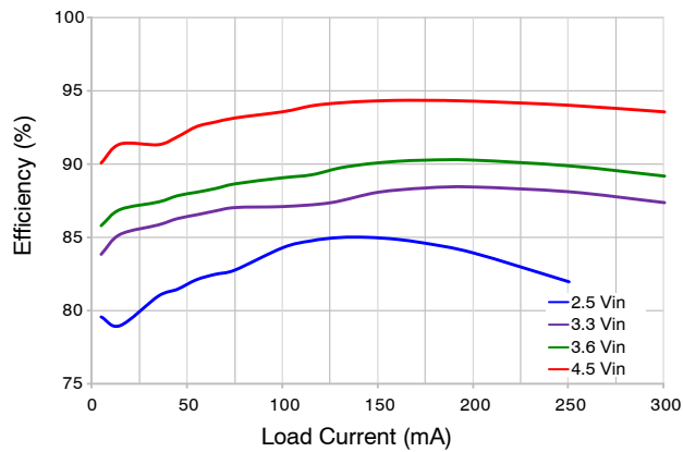
Figure 15. Efficiency vs. V IN
