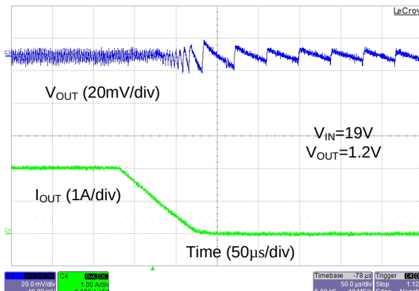
Figure 20. Operation as Load Changes from 2 A to 0 A
