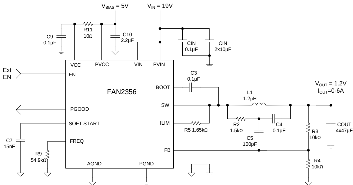
Figure 1. Typical Application
