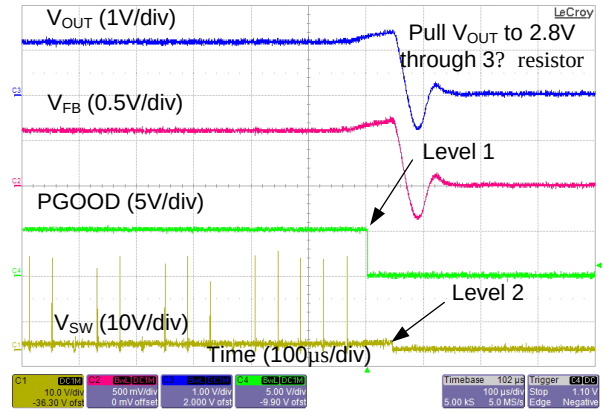
Figure 24. Over-Voltage Protection Level 1 and Level 2
