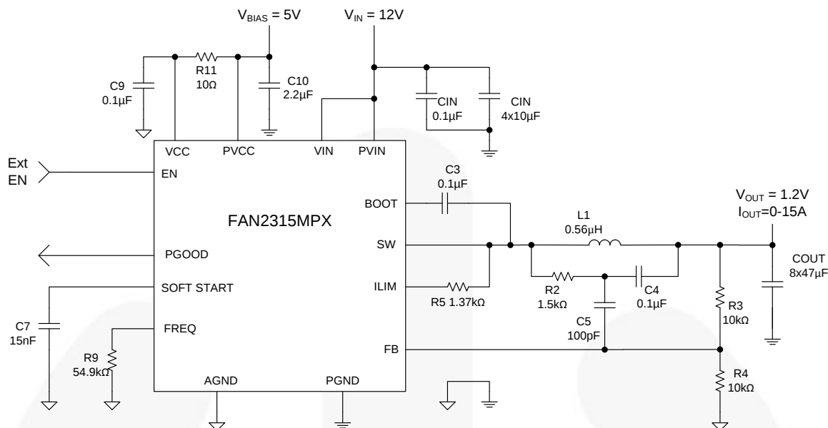
Figure 1. Typical Application
