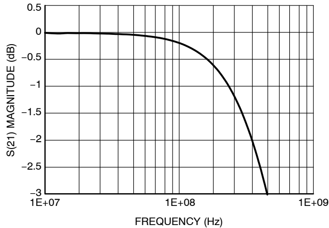
Figure 11. Insertion Loss
