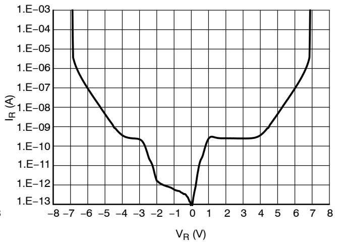
Figure 8. Reverse Leakage Current
