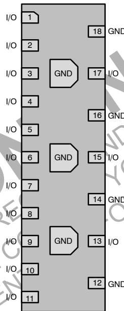
Figure 2. Pin Configuration
