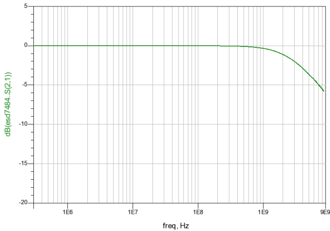
Figure 3. S21 Plot
