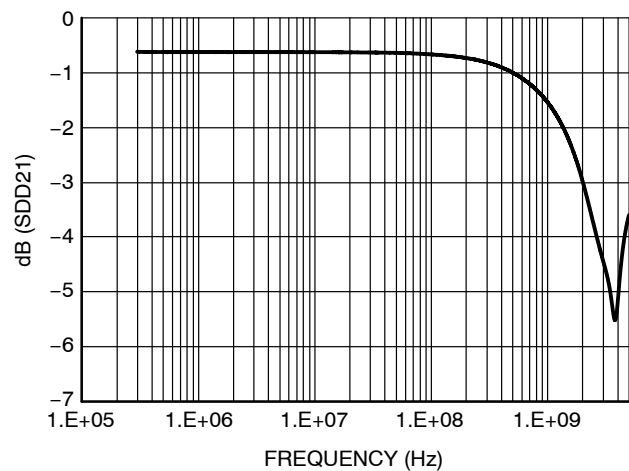
Figure 2. Typical Differential Mode Attenuation vs. Frequency
