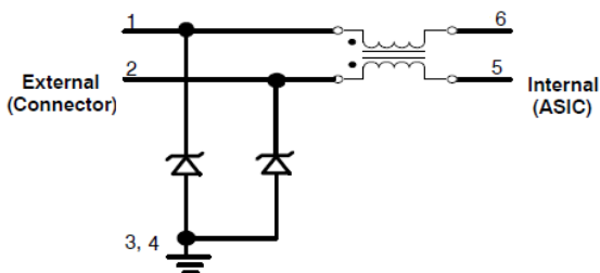
Figure 1. EMI8031 Electrical Schematic
