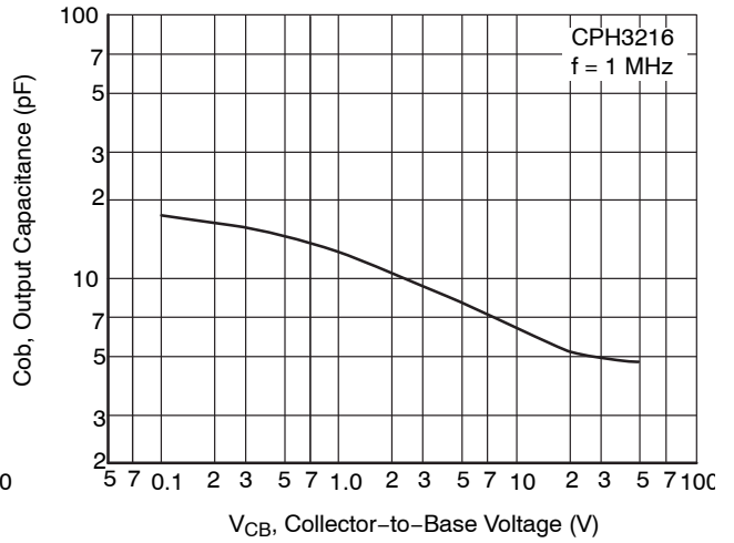
Figure 11. C_{ob} - V_{CB}
