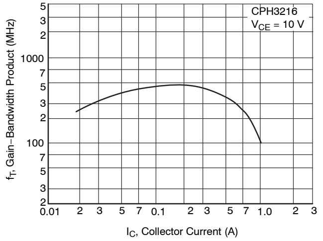
Figure 9. f_T - I_C
