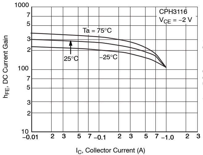
Figure 6. h_{FE} - I_C
