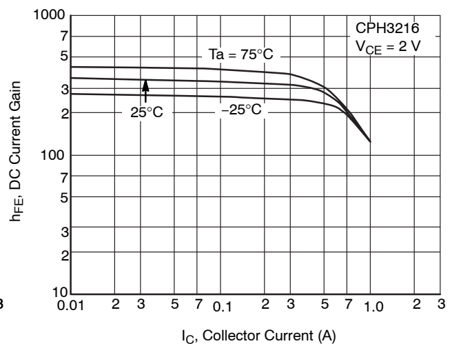
Figure 7. h_{FE} - I_C
