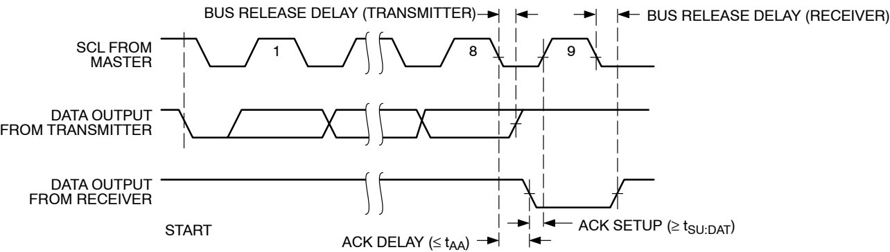
Figure 4. Acknowledge Timing
