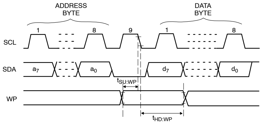
Figure 9. WP Timing
