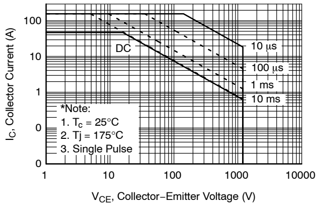
Figure 15. SOA Characteristics
