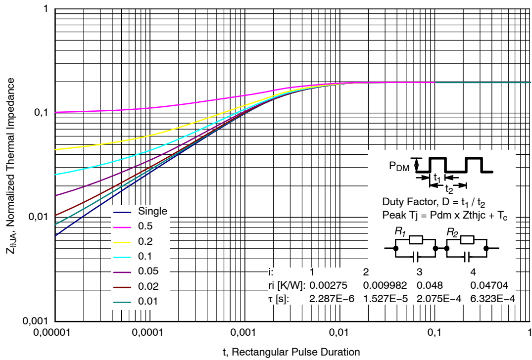
Figure 16. Transient Thermal Impedance of IGBT
