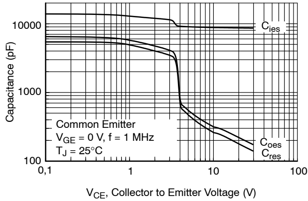
Figure 7. Capacitance Characteristics
