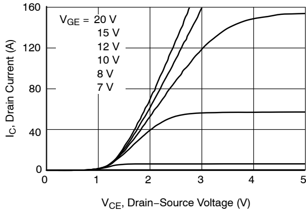
Figure 1. Typical Output Characteristics (25°C)
