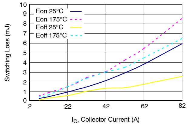
Figure 14. Switching Loss vs. Collector Current
