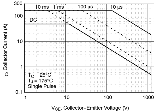
Figure 15. SOA Characteristics (FBSOA)
