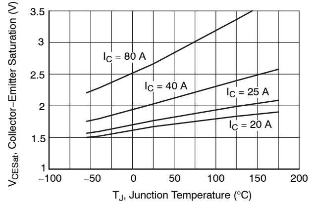
Figure 4. Saturation Voltage vs. Junction Temperature
