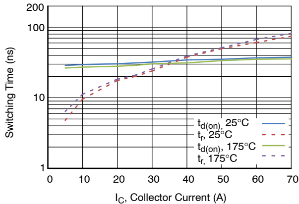
Figure 11. Turn-On Characteristics vs. Collector Current
