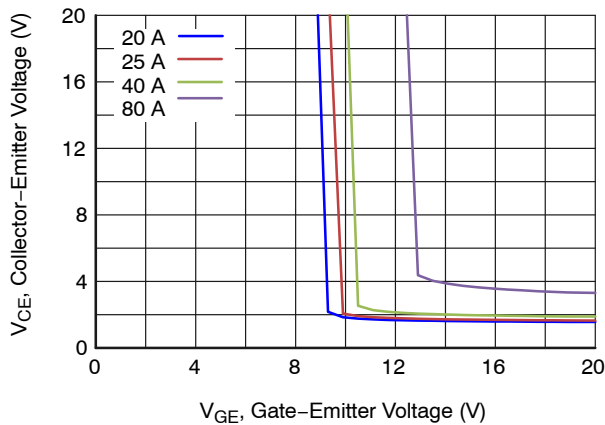
Figure 5. Saturation Voltage vs. V_{GE} (25°C)
