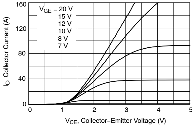
Figure 1. Typical Output Characteristics (25°C)
