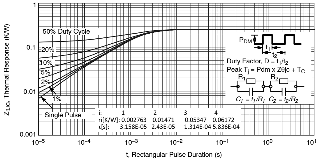
Figure 16. Transient Thermal Impedance of IGBT
