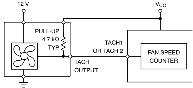
Figure 25. Fan with Tach Pull-up to + V_{\text{CC}}
