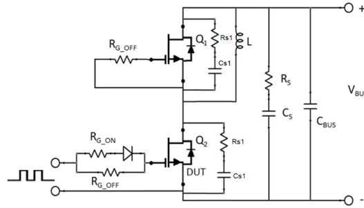
Figure 31. Schematic of the Half-Bridge Mode Switching Test Circuit with device RC Snubber ( R_{S1} = 10 \, \Omega , C_{S1} = 95 \, \text{nF} ) and a Bus RC Snubber ( R_S = 2.5 \, \Omega , C_S = 100 \, \text{nF} ).
