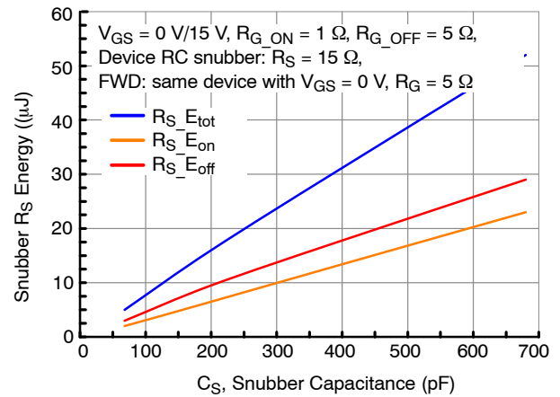
Figure 26. RC Snubber Energy Losses vs. Snubber Capacitance C_{\text{S}} at V_{\text{DS}} = 400 \text{ V} , I_{\text{D}} = 25 \text{ A} and T_{\text{J}} = 25 \text{ }^{\circ}\text{C}
