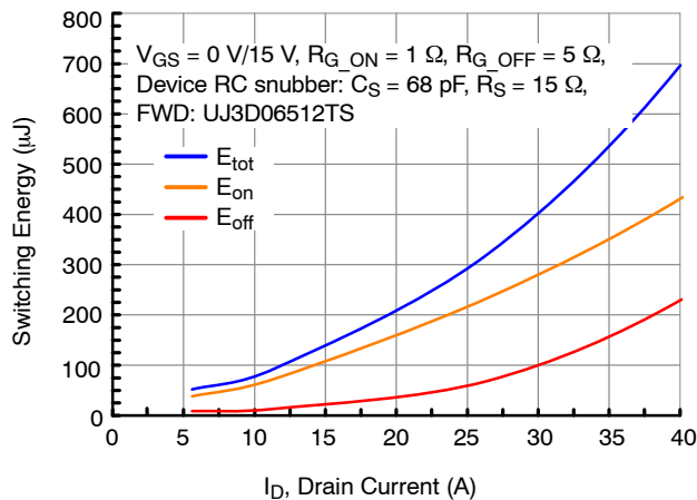
Figure 29. Clamped Inductive Switching Energy vs. Drain Current at V_{\text{DS}} = 400 \text{ V} and T_{\text{J}} = 25 \text{ }^{\circ}\text{C}
