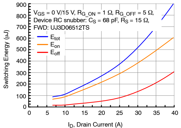
Figure 30. Clamped Inductive Switching Energy vs. Drain Current at V_{\text{DS}} = 500 \text{ V} and T_{\text{J}} = 25 \text{ }^{\circ}\text{C}
