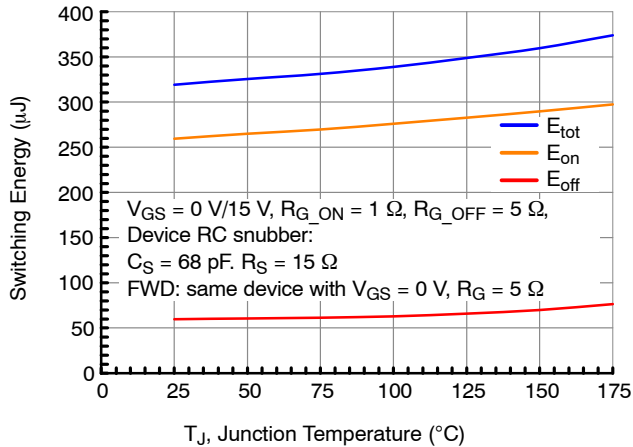
Figure 27. Clamped Inductive Switching Energy vs. Junction Temperature at V_{\text{DS}} = 400 \text{ V} and I_{\text{D}} = 25 \text{ A}
