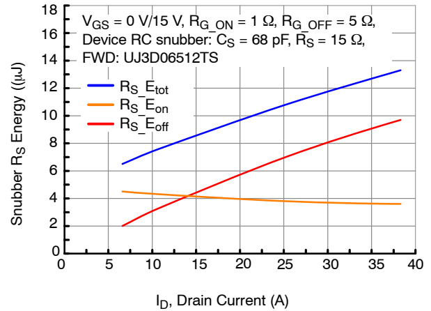
Figure 32. RC Snubber Energy Losses vs. Drain Current at V_{DS} = 500 V and T_J = 25 °C
