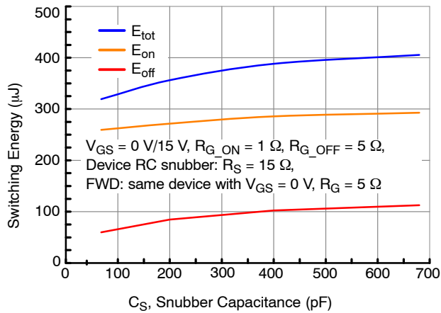
Figure 25. Clamped Inductive Switching Energies vs. Snubber Capacitance C_{\text{S}} at V_{\text{DS}} = 400 \text{ V} , I_{\text{D}} = 25 \text{ A} and T_{\text{J}} = 25 \text{ }^{\circ}\text{C}
