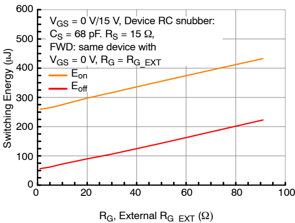
Figure 23. Clamped Inductive Switching Energies vs. R_{G\_EXT} at V_{DS} = 400 V, I_D = 25 A and T_J = 25 °C
