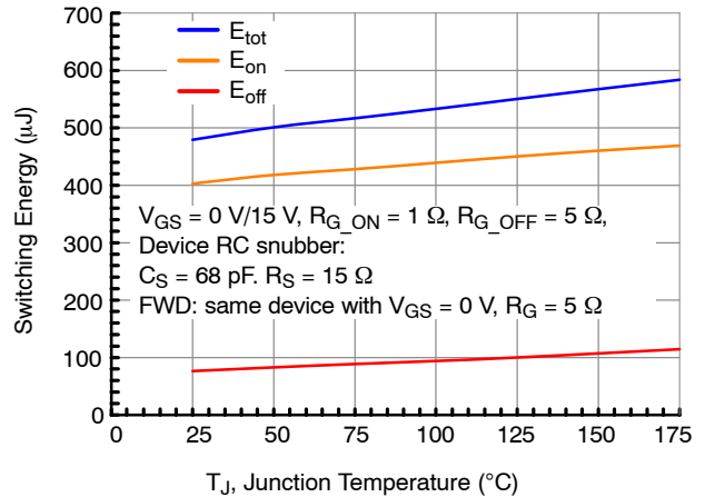
Figure 28. Clamped Inductive Switching Energy vs. Junction Temperature at V_{\text{DS}} = 500 \text{ V} , I_{\text{D}} = 25 \text{ A}
