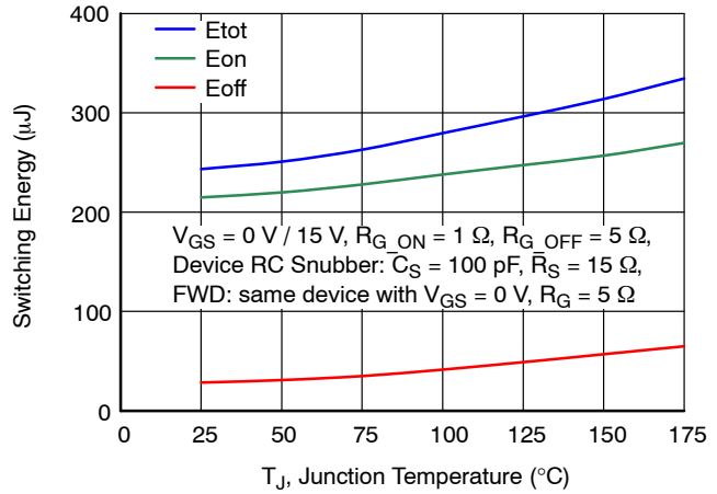
Figure 28. Clamped Inductive Switching Energy vs. Junction Temperature at V_{DS} = 500 V and I_D = 30 A
