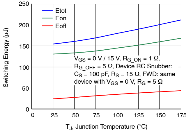
Figure 27. Clamped Inductive Switching Energy vs. Junction Temperature at V_{DS} = 400 V and I_D = 30 A
