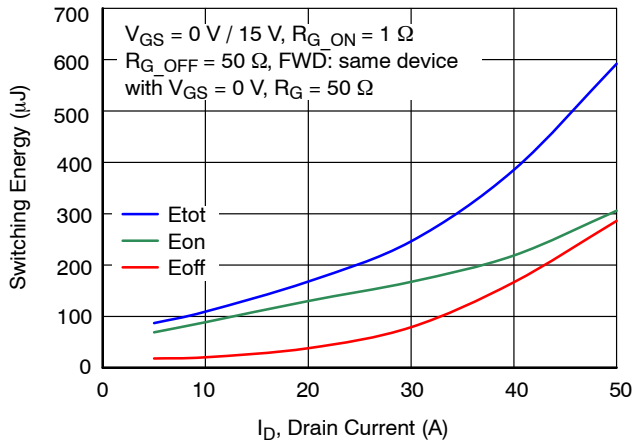
Figure 19. Clamped Inductive Switching Energies vs. Drain Current at V_{DS} = 400 V and T_J = 25 °C
