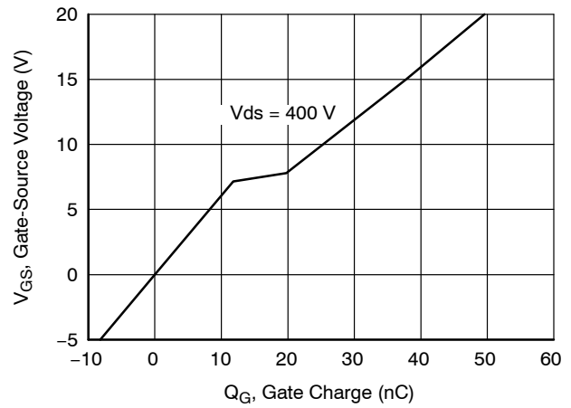
Figure 8. Typical Gate Charge I_D = 40\text{ A}
