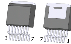
TO-263-7 10.18x9.08x4.43, 1.27P CASE 418BA
