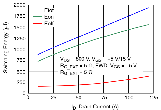
Figure 18. Clamped Inductive Switching Energy vs. Drain Current at T_J = 25 °C
