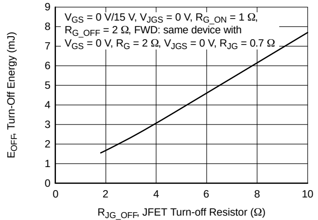
Figure 20. Clamped Inductive Turn-Off Energy vs. JFET Gate Resistor R_{JG\_OFF} at V_{DS} = 800\text{ V} , I_D = 100\text{ A} , and T_J = 25\text{ °C}
