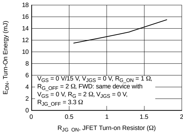
Figure 21. Clamped Inductive Switching Turn-On Energy vs. JFET Gate Resistor R_{JG\_ON} at V_{DS} = 800\text{ V} , I_D = 100\text{ A} , and T_J = 25\text{ °C}
