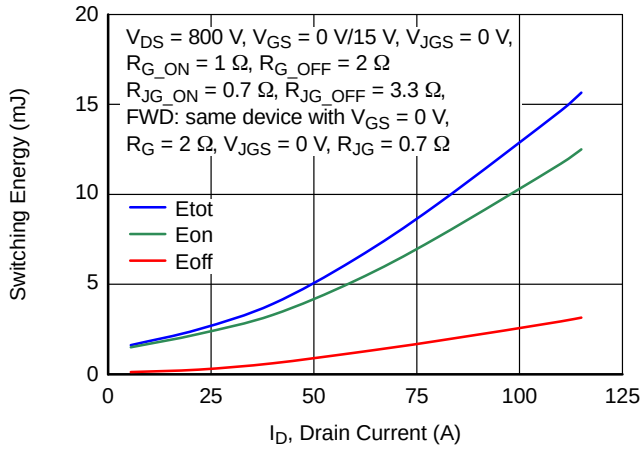
Figure 19. Clamped Inductive Switching Energy vs. Drain Current at T_J = 25\text{ °C}
