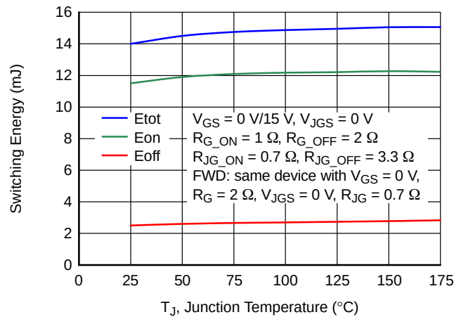
Figure 22. Clamped Inductive Switching Energy vs. Junction Temperature at V_{DS} = 800\text{ V} and I_D = 100\text{ A}
