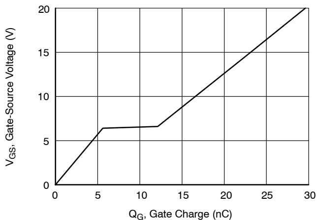
Figure 8. Typical Gate Charge at V_{DS} = 1200\text{ V} and I_D = 5\text{ A}
