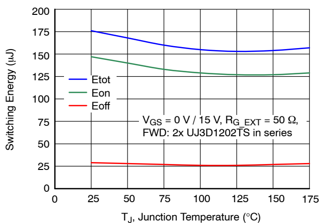
Figure 20. Clamped Inductive Switching Energy vs. Junction Temperature at V_{DS} = 1200 \text{ V} , and I_D = 5 \text{ A}
