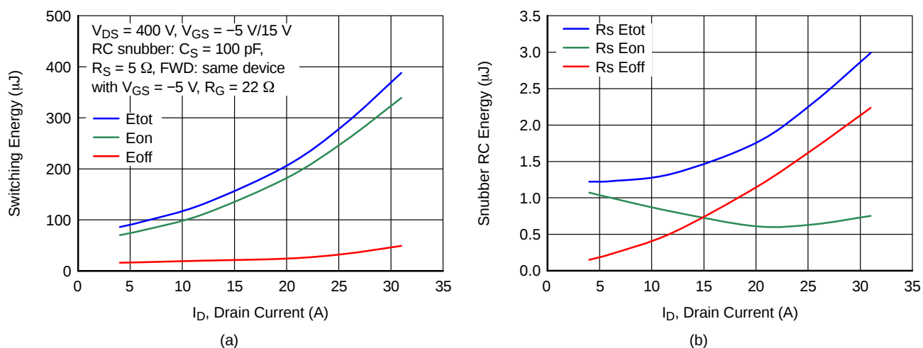
Figure 19. Clamped Inductive Switching Energy (a) and RC Snubber Energy Loss (b) vs. Drain Current at T_J = 25 ^{\circ} C, Turn-On R_{G\_EXT} = 1 \Omega , and Turn-off R_{G\_EXT} = 22 \Omega
