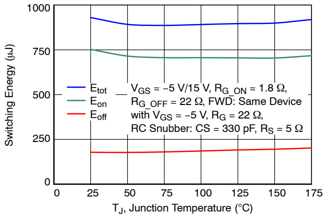
Figure 25. Clamped Inductive Switching Energy Including RC Snubber Energy Loss as a Function of Junction Temperature at I_D = 50 \text{ A} and V_{\text{DS}} = 400 \text{ V}
