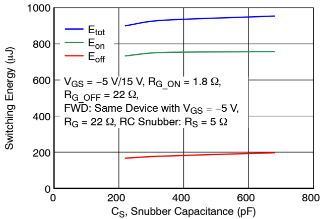
Figure 27. Clamped Inductive Switching Energy Including RC Snubber Energy Loss as a Function of Snubber Capacitance at I_D = 50 \text{ A} , V_{\text{DS}} = 400 \text{ V} , and T_J = 25 \text{ }^{\circ}\text{C}
