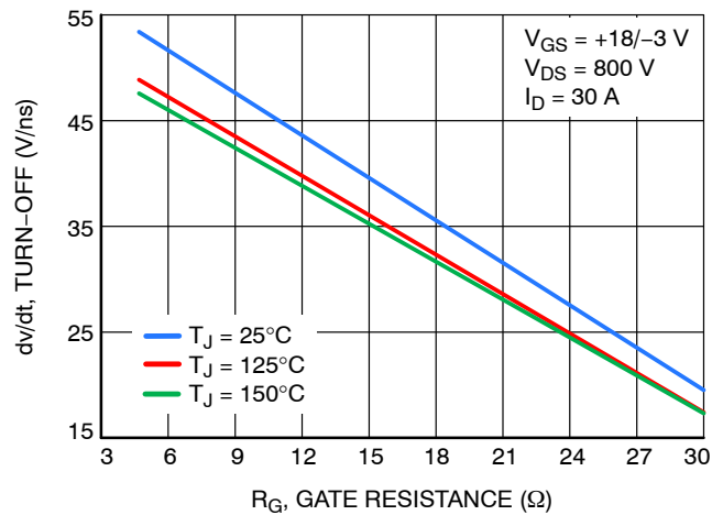
Figure 24. \frac{dv}{dt} Turn OFF vs. Gate Resistance V_{DS} = 800 V
