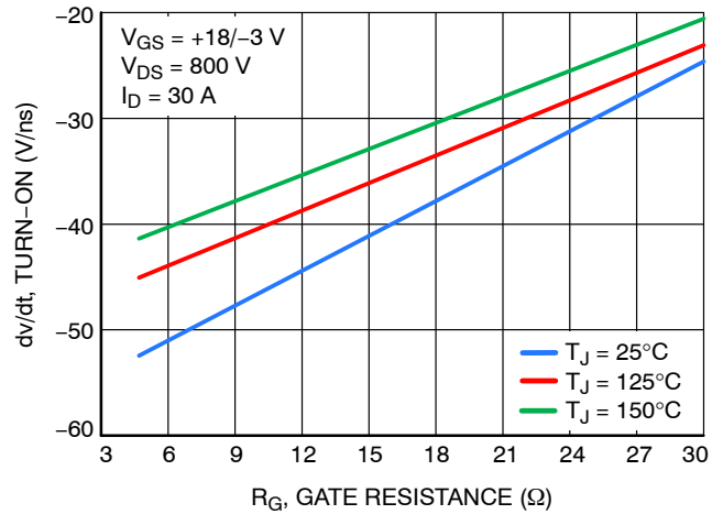
Figure 22. \frac{dv}{dt} Turn ON vs. Gate Resistance V_{DS} = 800 V
