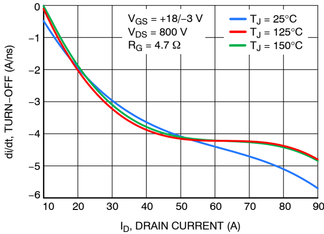
Figure 19. \frac{di}{dt} Turn OFF vs. Drain Current V_{DS} = 800 V
