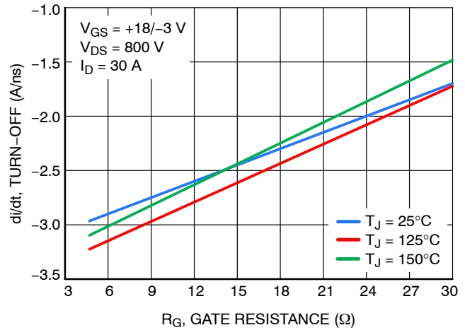
Figure 20. \frac{di}{dt} Turn OFF vs. Gate Resistance V_{DS} = 800 V
