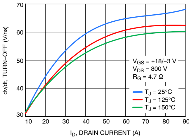
Figure 23. \frac{dv}{dt} Turn OFF vs. Drain Current V_{DS} = 800 V
