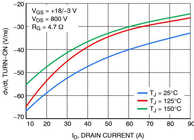
Figure 21. \frac{dv}{dt} Turn ON vs. Drain Current V_{DS} = 800 V
