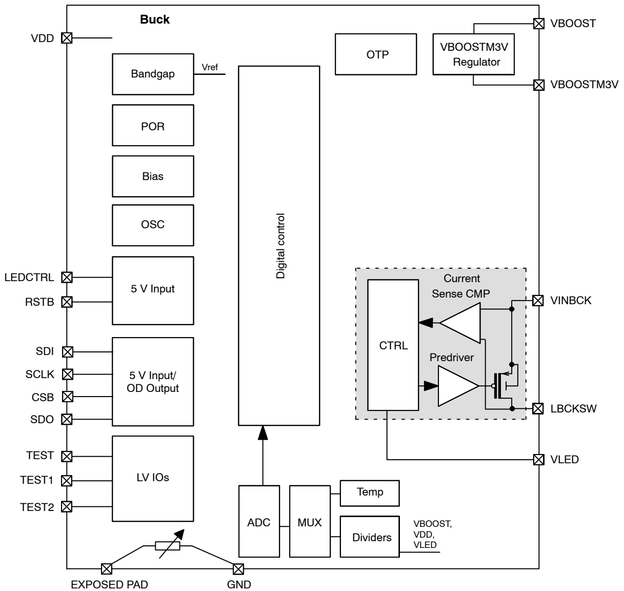
Figure 2. Block Diagram
