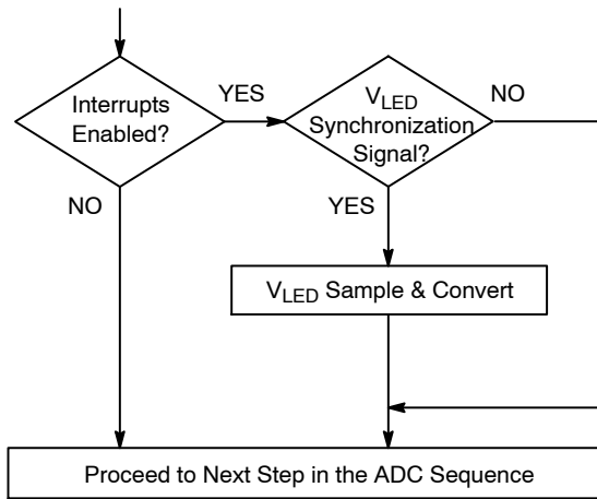
Figure 15. ADC VLED Interrupt Sequence
