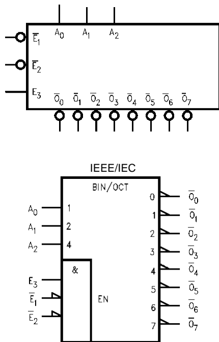
Figure 1. Logic Symbols
