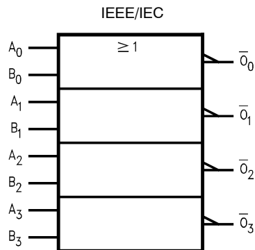
Figure 1. Logic Symbol
