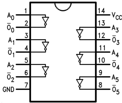
Figure 1. Connection Diagram
