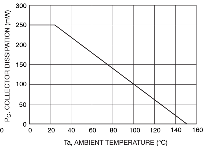
Figure 10. P_C – T_a
