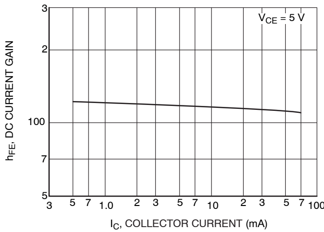
Figure 3. h_{FE} - I_C
