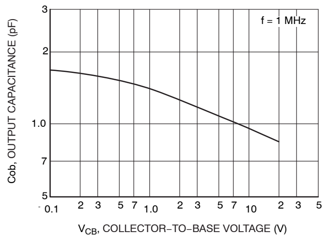
Figure 5. C_{ob} - V_{CB}
