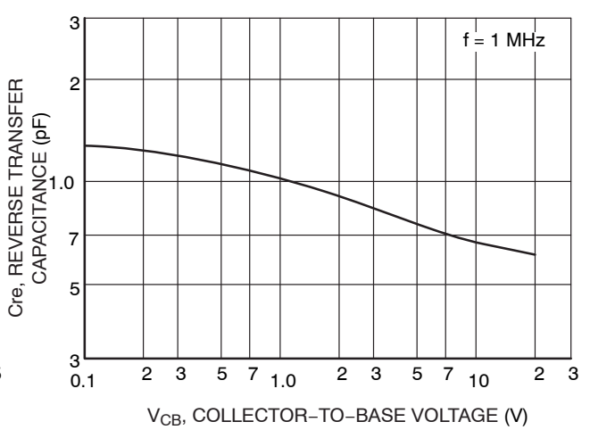
Figure 6. C_{re} - V_{CB}
