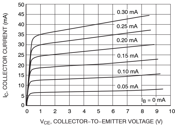
Figure 1. I_C - V_{CE}
