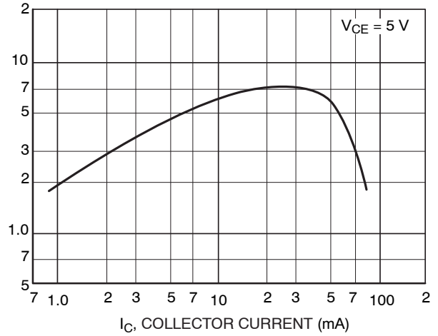
Figure 2. f_T - I_C
