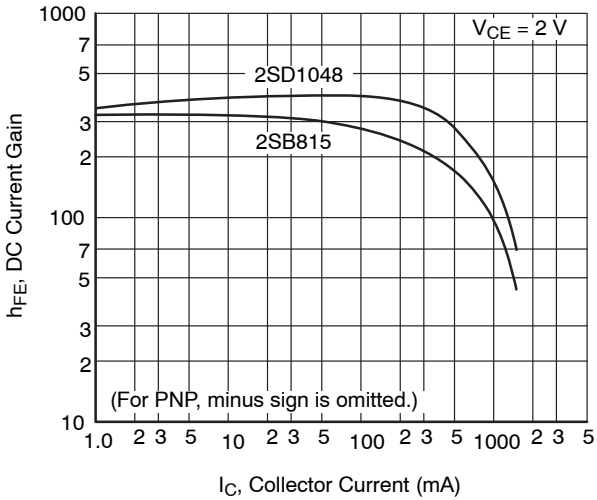
Figure 5. h_{FE} - I_C
