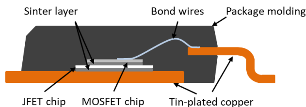
Figure 1. D2PAK-7L Cross-Section Drawing of a onsemi Cascode, Not to Scale, JFET Gate Bond Wire Omitted for Clarity
