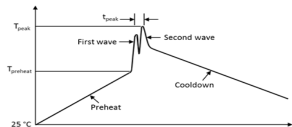
Figure 2. Typical Dual-Wave solder Profile
