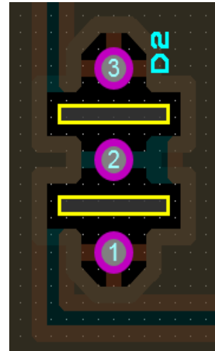
Figure 3. Example of Thermal Relief “Spokes” to TO-247 Leads, with Slots Between Leads to Increase Creepage Distance
