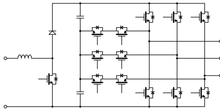
Figure 6. Booster Paired with TNPC Inverter
