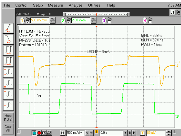
Figure 2. Switching Performance with Peak LED Current at 3 mA
