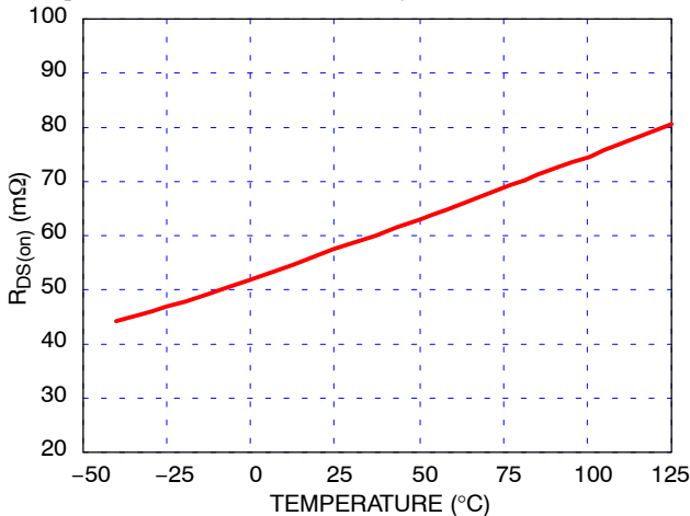
Figure 13. Typical R DS(on) versus Temperature
