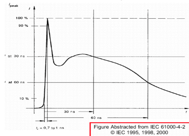
Figure 14. IEC 61000-4-2 Electrostatic Discharge
