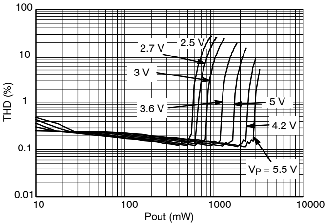
Figure 5. NCP2823B, THD+N vs P_{out} , R_L = 4 \Omega
