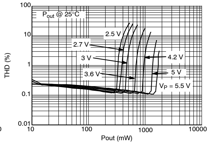
Figure 4. NCP2823A, THD+N vs P_{out} , R_L = 8 \Omega
