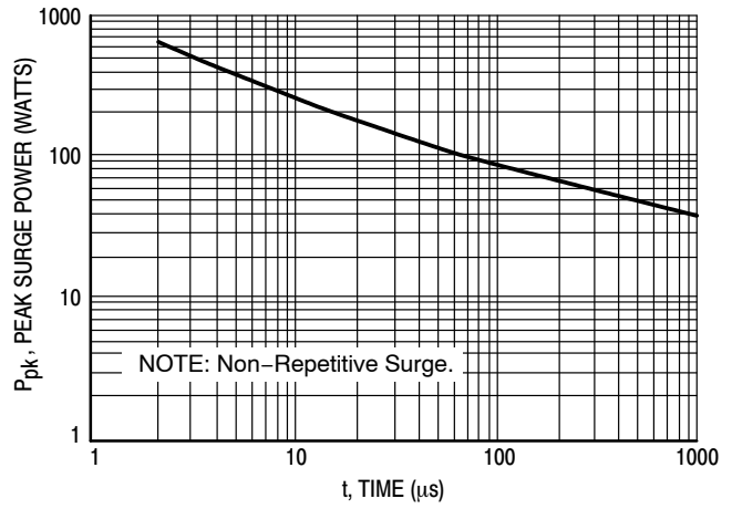
Figure 9. Pulse Width
